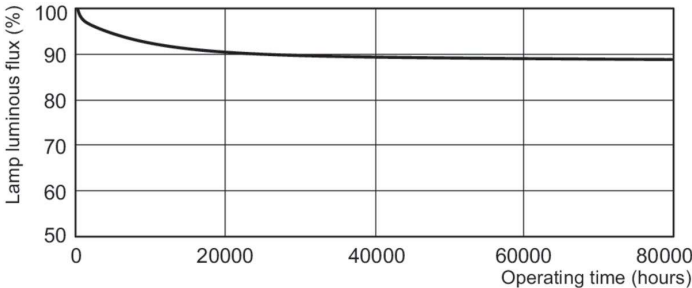
Lumen Maintenance Diagram - MASTER TL5 HO Xtra 80W/840 SLV/20
