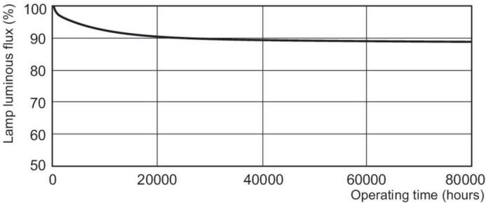
Lumen Maintenance Diagram - MASTER TL5 HO Xtra 80W/840 SLV/20
