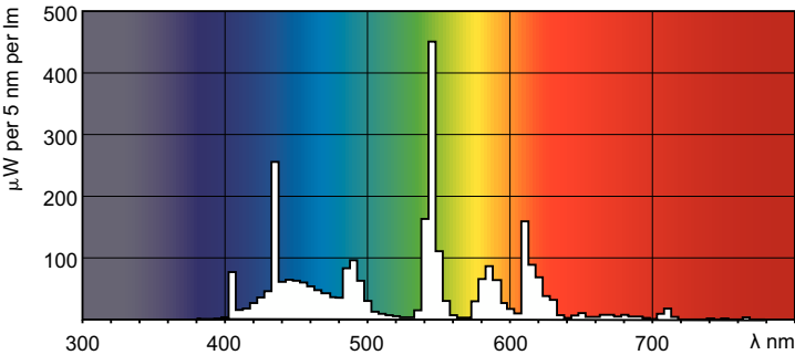
Spectral Power Distribution Colour - PL-L Essential 55W/865/4P 1CT/50
