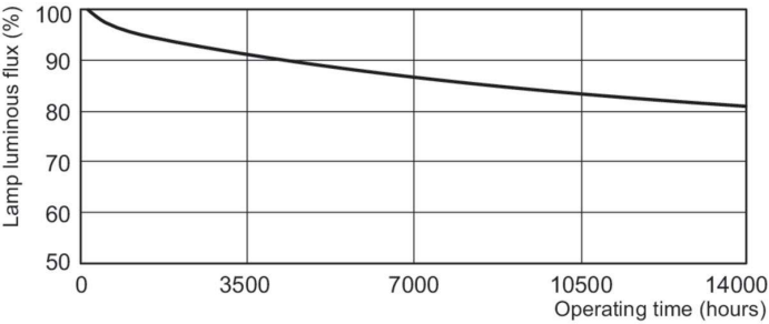
Lumen Maintenance Diagram - MASTER PL-S 5W/840/2P 1CT/5X10BOX
