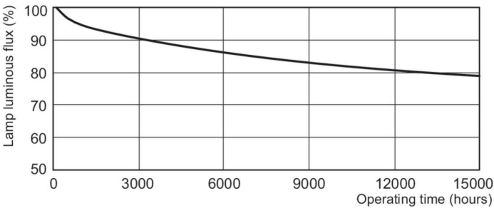
Lumen Maintenance Diagram - MASTER PL-S 7W/830/4P 1CT/5X10BOX
