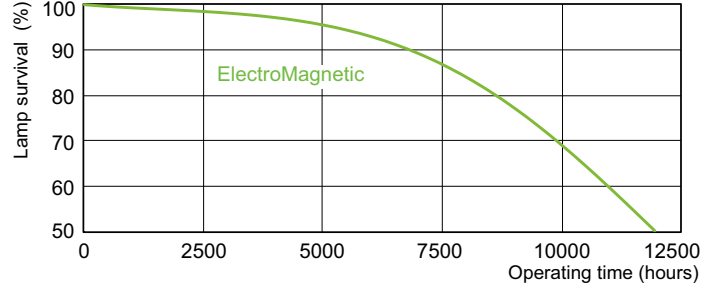
Life Expectancy Diagram - PL-Q 16W/827/2P 1CT/10BOX
