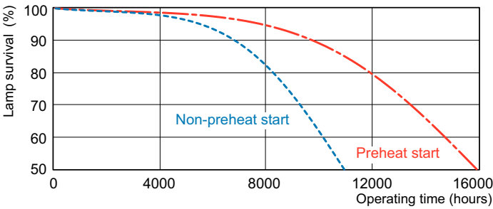
Life Expectancy Diagram - MASTER TL5 Circular 55W/865 1CT/10
