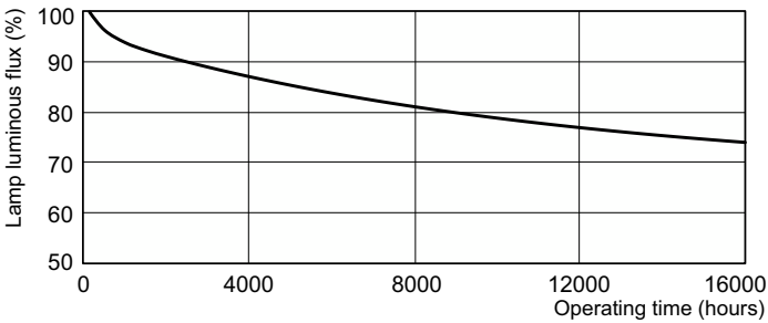
Lumen Maintenance Diagram - MASTER TL5 Circular 55W/865 1CT/10
