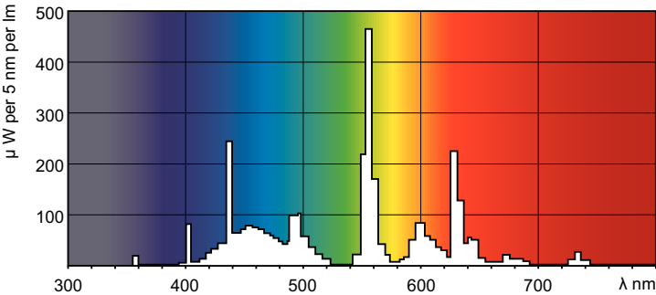
Spectral Power Distribution Colour - MASTER TL5 Circular 55W/865 1CT/10
