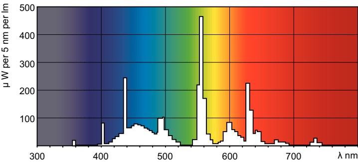
Spectral Power Distribution Colour - MASTER TL-D Xtra 18W/865 SLV
