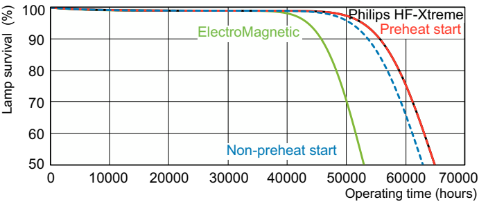
Life Expectancy Diagram - MASTER TL-D Xtra Secura 36W/840 SLV/25
