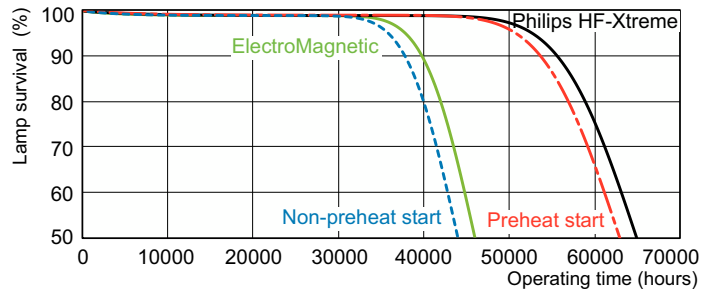
Life Expectancy Diagram - MASTER TL-D Xtra Polar 58W/840 T12 SLV
