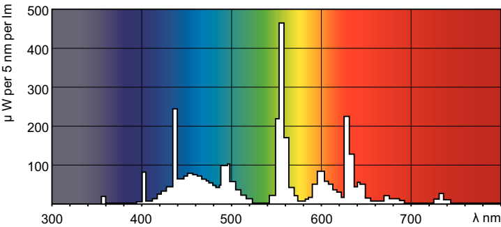
Spectral Power Distribution Colour - MASTER TL5 HE Eco 13=14W/865 1SL/40
