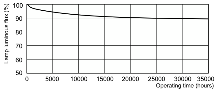
Lumen Maintenance Diagram - MASTER TL5 HO Eco 20=24W/840 1SL/40
