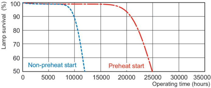
Life Expectancy Diagram - F28T5 841 HE EA ALTO 25W
