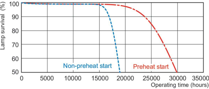
Life Expectancy Diagram - F28T5 850 HE EA ALTO 25W
