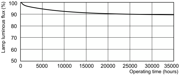
Lumen Maintenance Diagram - F28T5 850 HE EA ALTO 25W
