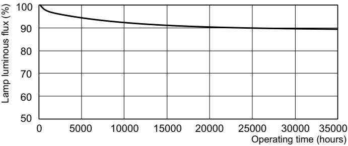
Lumen Maintenance Diagram - MASTER TL5 HO Eco 73=80W/830 1SL/40
