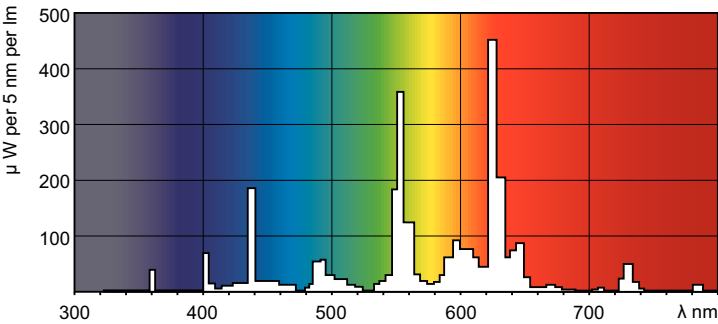
Spectral Power Distribution Colour - MASTER TL5 HO Eco 73=80W/830 1SL/40
