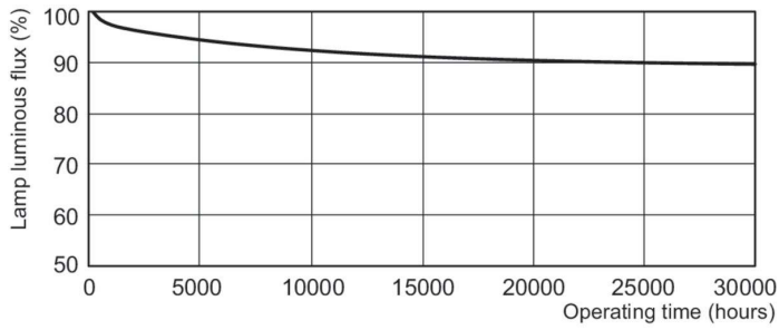
Lumen Maintenance Diagram - MASTER TL5 HO 90 De Luxe 24W/965 1SL20
