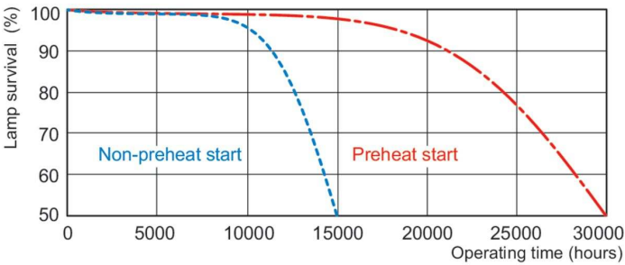
Life Expectancy Diagram - F54T5/835/HO/XEW/ALTO/44W
