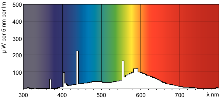
Spectral Power Distribution Colour - TL Mini 6W/33-640 1PP/10
