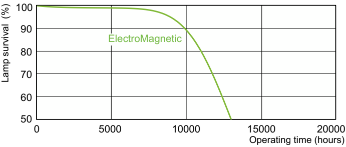
Life Expectancy Diagram - F15T8/D 25PK
