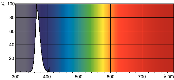
Spectral Power Distribution Colour - F15T8/BLACKLIGHT/18 BLB LF6PK
