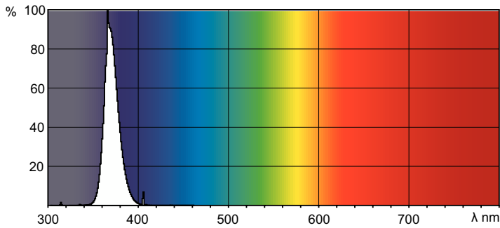
Spectral Power Distribution Colour - F15T8/BLACKLIGHT/18 BLB LF6PK
