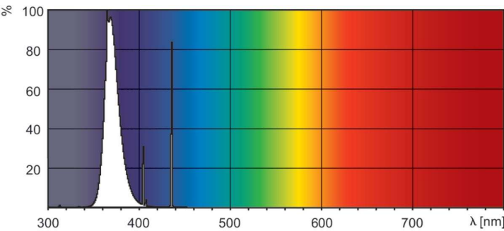
Spectral Power Distribution Colour - MASTER Actinic BL TL-D 18W/10 Secura
