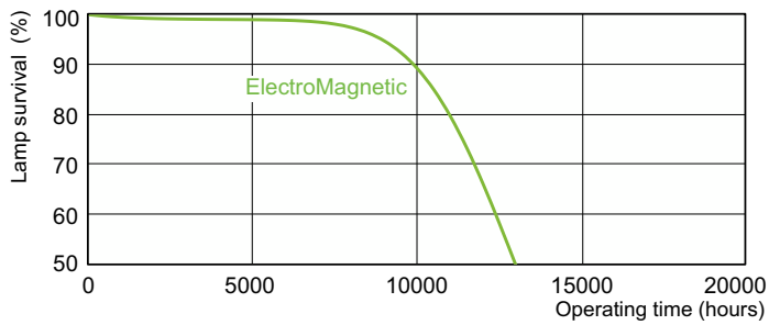
Life Expectancy Diagram - TL-D 18W/29-530 1SL/25
