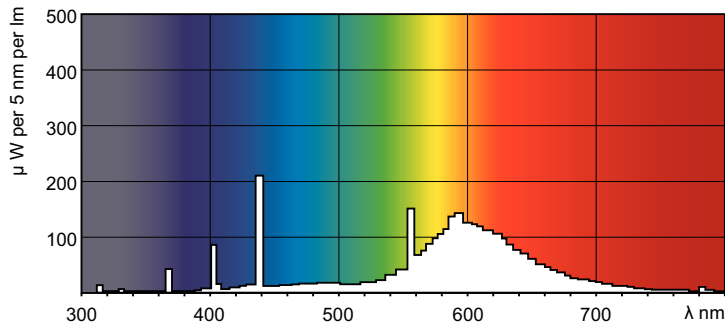
Spectral Power Distribution Colour - TL-D 18W/29-530 1SL/25
