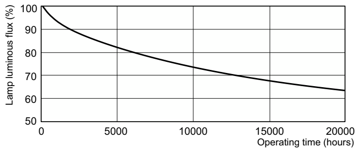
Lumen Maintenance Diagram - TL-D 18W/29-530 1SL/25
