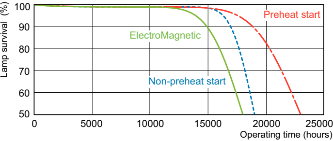
Life Expectancy Diagram - MST TL-D Reflex 36W/865 1 SLV/25
