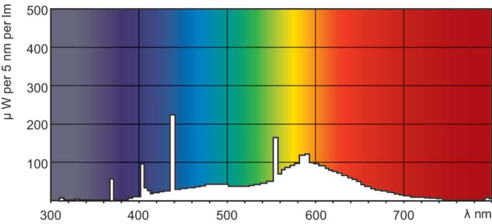
Spectral Power Distribution Colour - TL-D 36W/33-640 UNP/25
