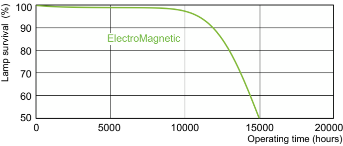
Life Expectancy Diagram - TL-D 36W/33-640 UNP/25
