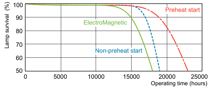
Life Expectancy Diagram - MST TL-D Reflex 58W/840 1 SLV/25
