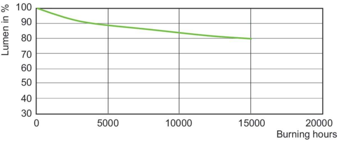
Lumen Maintenance Diagram - MC CDM-R Elite 35W/930 E27 PAR20 10D
