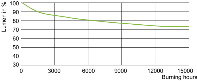
Lumen Maintenance Diagram - MC CDM-R Elite 35W/942 E27 PAR20 10D
