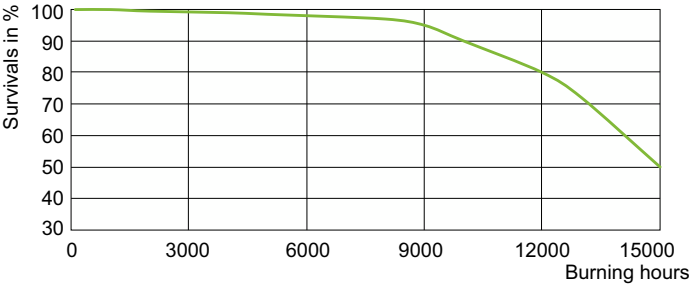
Life Expectancy Diagram - MC CDM-R Elite 35W/942 E27 PAR20 10D
