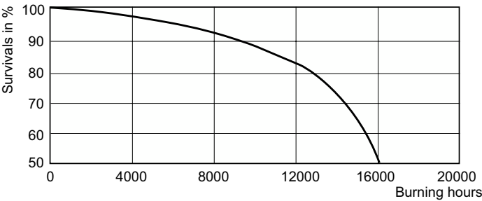
Life Expectancy Diagram - HPL-N 80W E27 SG 1CT/24
