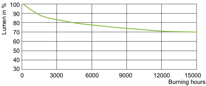
Lumen Maintenance Diagram - MC CDM-R Elite 35W/942 E27 PAR30L 30D
