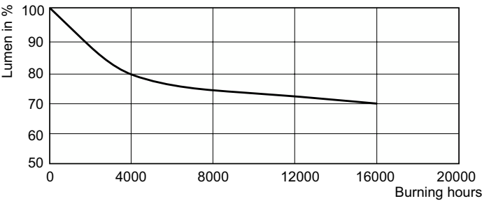
Lumen Maintenance Diagram - HPL-N 125W/542 E27 SG 1CT/24
