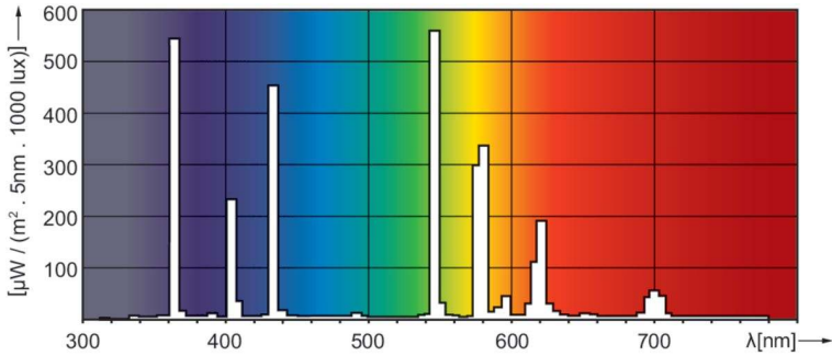
Spectral Power Distribution Colour - HPL-N 125W/542 E27 SG 1CT/24
