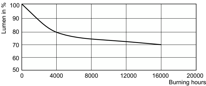
Lumen Maintenance Diagram - HPL-N 250W E40 HG SLV/12
