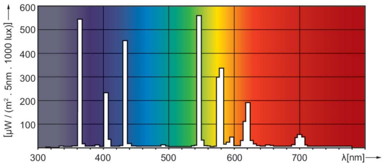
Spectral Power Distribution Colour - HPL-N 400W E40 HG 1CT/6
