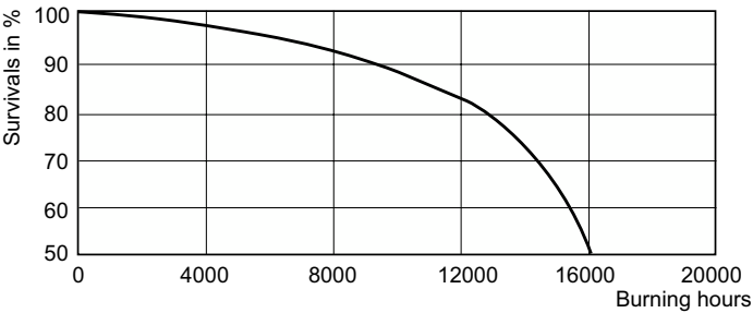
Life Expectancy Diagram - HPL-N 400W E40 HG 1CT/6
