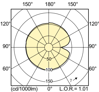
Light Distribution Diagram - MST CosmoWhite CPO-TT Xtra 45W/628 E27
