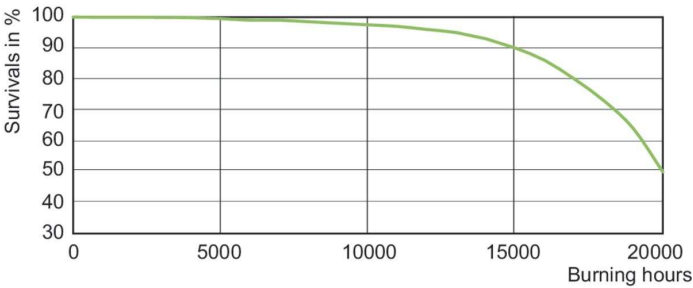
Life Expectancy Diagram - MC CDM-TC Evolution 70W/930 G8.5
