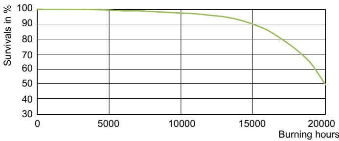
Life Expectancy Diagram - MC CDM-T Evolution 70W/930 G12
