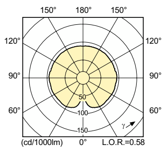
Light Distribution Diagram - MC CDM-TC Evolution 20W/930 G8.5
