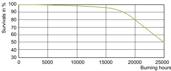
Life Expectancy Diagram - MC CDM-TC Evolution 20W/930 G8.5
