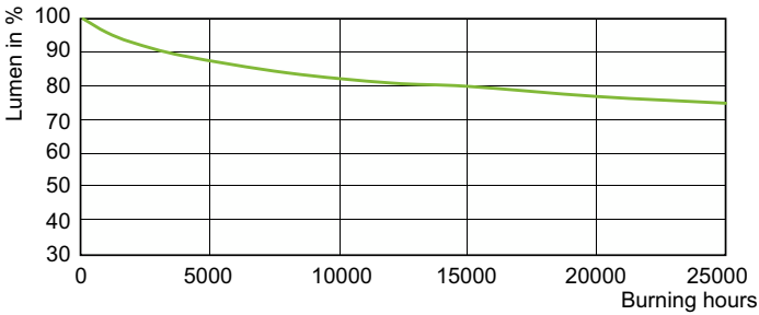
Lumen Maintenance Diagram - MC CDM-TC Evolution 20W/930 G8.5
