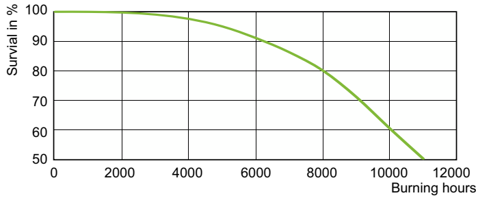
Life Expectancy Diagram - MASTERC CDM-R 35W/830 E27 PAR30L 30D 1CT
