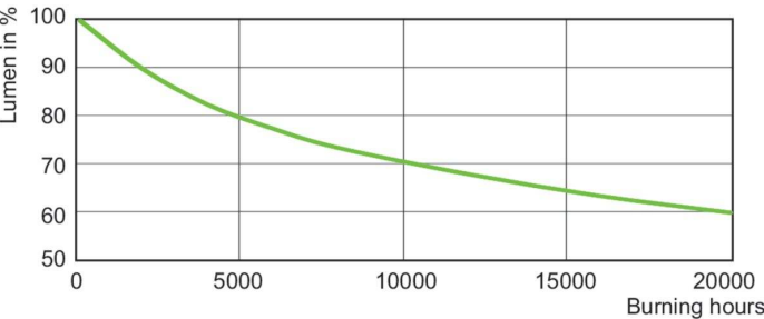
Lumen Maintenance Diagram - HPI PLUS 400W/667 BU E40 1SL/6
