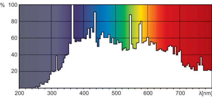
Spectral Power Distribution Colour - MSR 400 1CT/4
