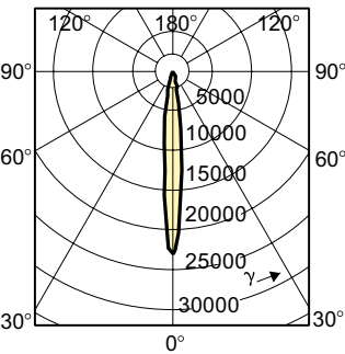
Light Distribution Diagram - MASTERC CDM-R 35W/830 E27 PAR20 10D 1CT
