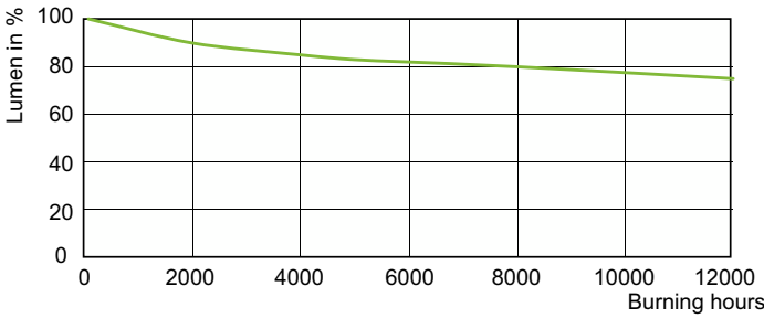
Lumen Maintenance Diagram - MASTERC CDM-R 70W/942 E26 PAR30L 10D 1CT
