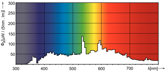
Spectral Power Distribution Colour - MASTERC CDM-R 70W/942 E26 PAR30L 10D 1CT
