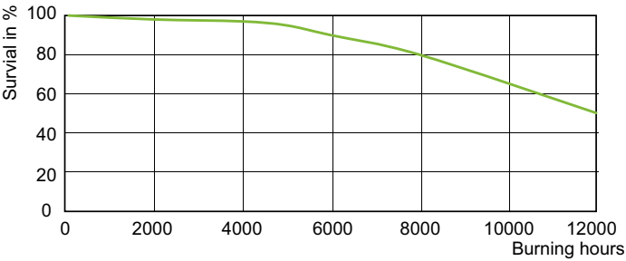
Life Expectancy Diagram - MASTERC CDM-R 70W/942 E26 PAR30L 10D 1CT
