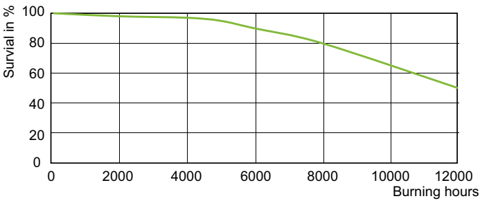
Life Expectancy Diagram - MASTERC CDM-R 70W/942 E27 PAR30L 10D 1CT
