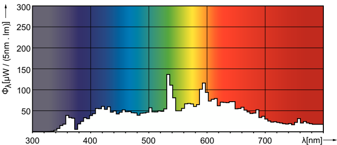
Spectral Power Distribution Colour - MASTERC CDM-R 70W/942 E27 PAR30L 10D 1CT
