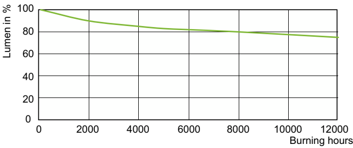
Lumen Maintenance Diagram - MASTERC CDM-R 70W/942 E27 PAR30L 10D 1CT
