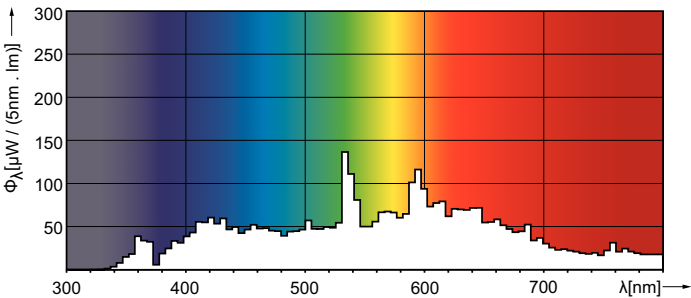
Spectral Power Distribution Colour - MASTERC CDM-R 35W/942 E26 PAR20 30D 1CT
