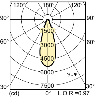
Light Distribution Diagram - MASTERC CDM-R 35W/942 E26 PAR20 30D 1CT
