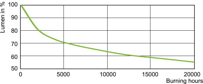
Lumen Maintenance Diagram - MASTERC CDM-TT 70W/942 E27 1SL/12
