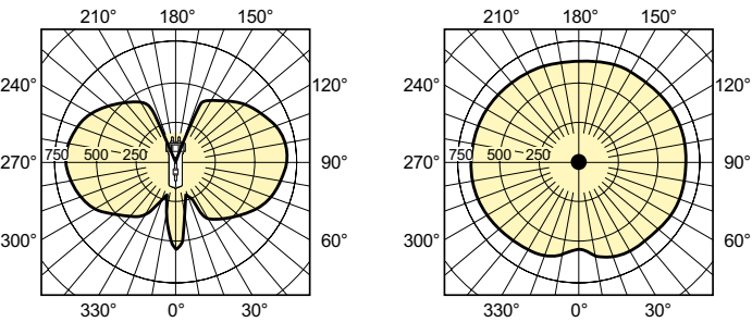
Light Distribution Diagram - MASTERC CDM-TT 70W/942 E27 1SL/12
