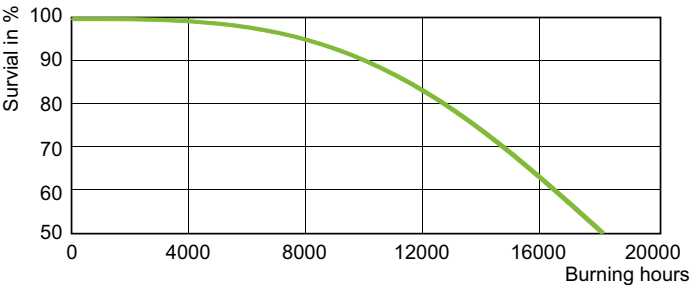
Life Expectancy Diagram - MASTERC CDM-TT 70W/942 E27 1SL/12
