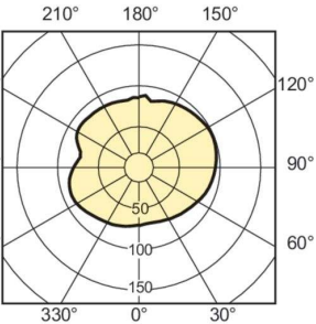
Light Distribution Diagram - MASTERC CDM-T 35W/842 G12 1CT/12
