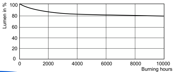
Lumen Maintenance Diagram - ML 250W E27 225-235V SG 1SL/12
