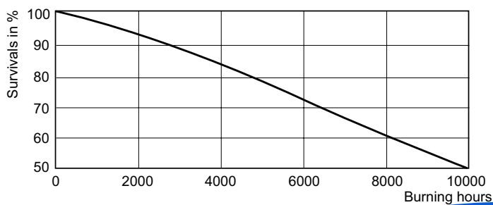
Life Expectancy Diagram - ML 250W E27 225-235V SG 1SL/12
